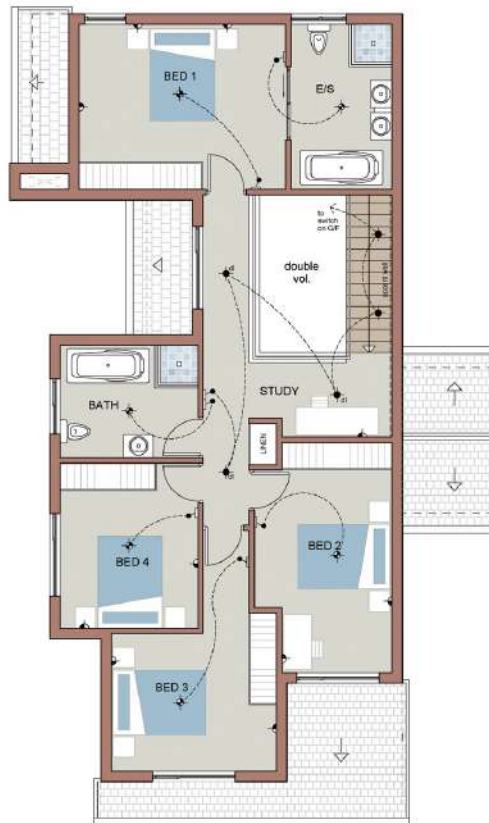
FIRST STOREY
