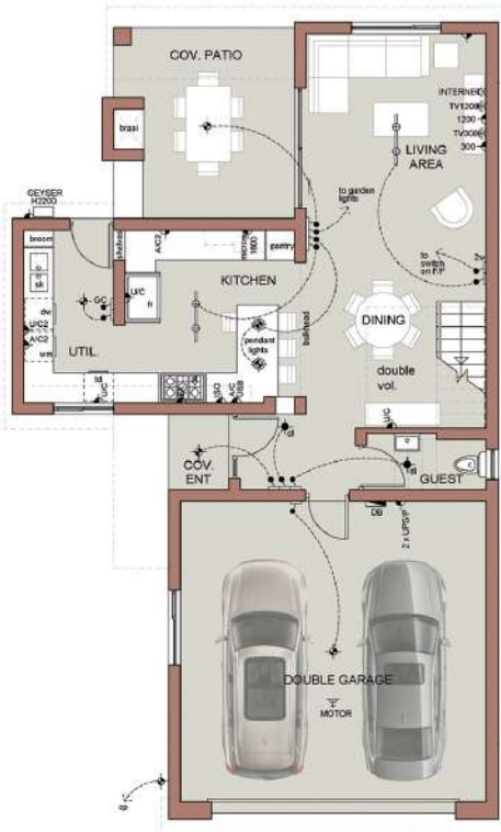
GROUND STOREY
