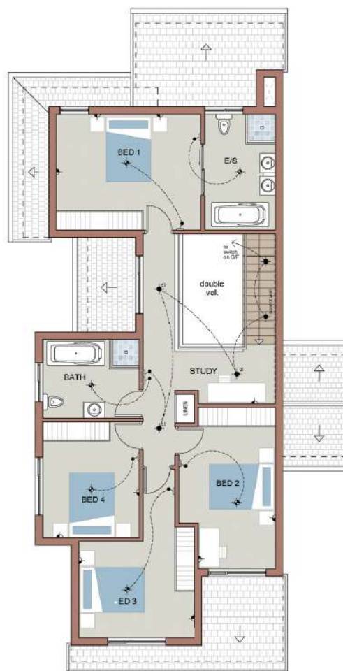
FIRST STOREY
