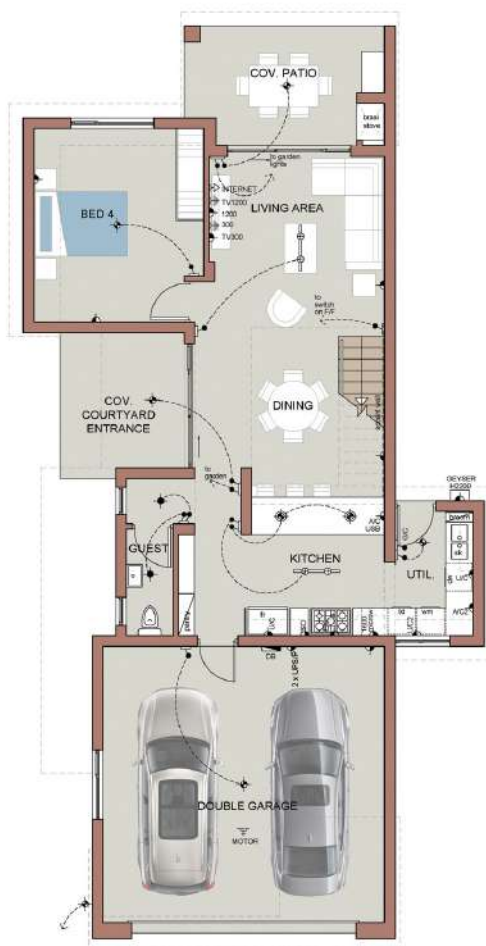
GROUND STOREY
