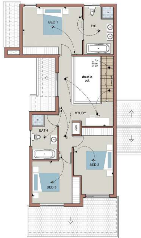
FIRST STOREY
