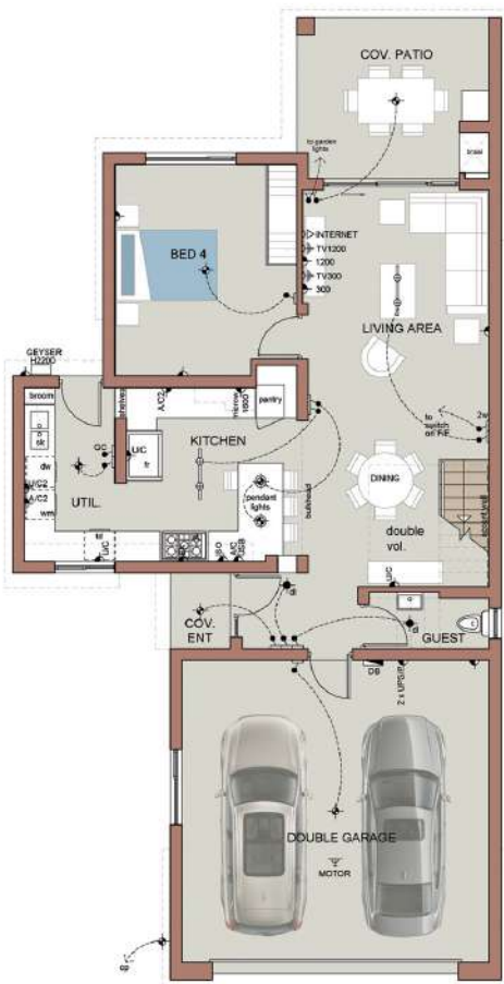
GROUND STOREY
